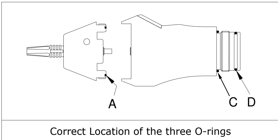
Nosecone O-ring Location
